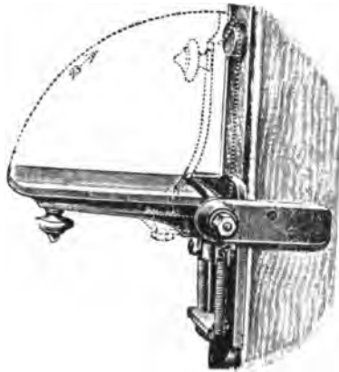
FIG. 49.—Automatic Closing Step (Section 192).
